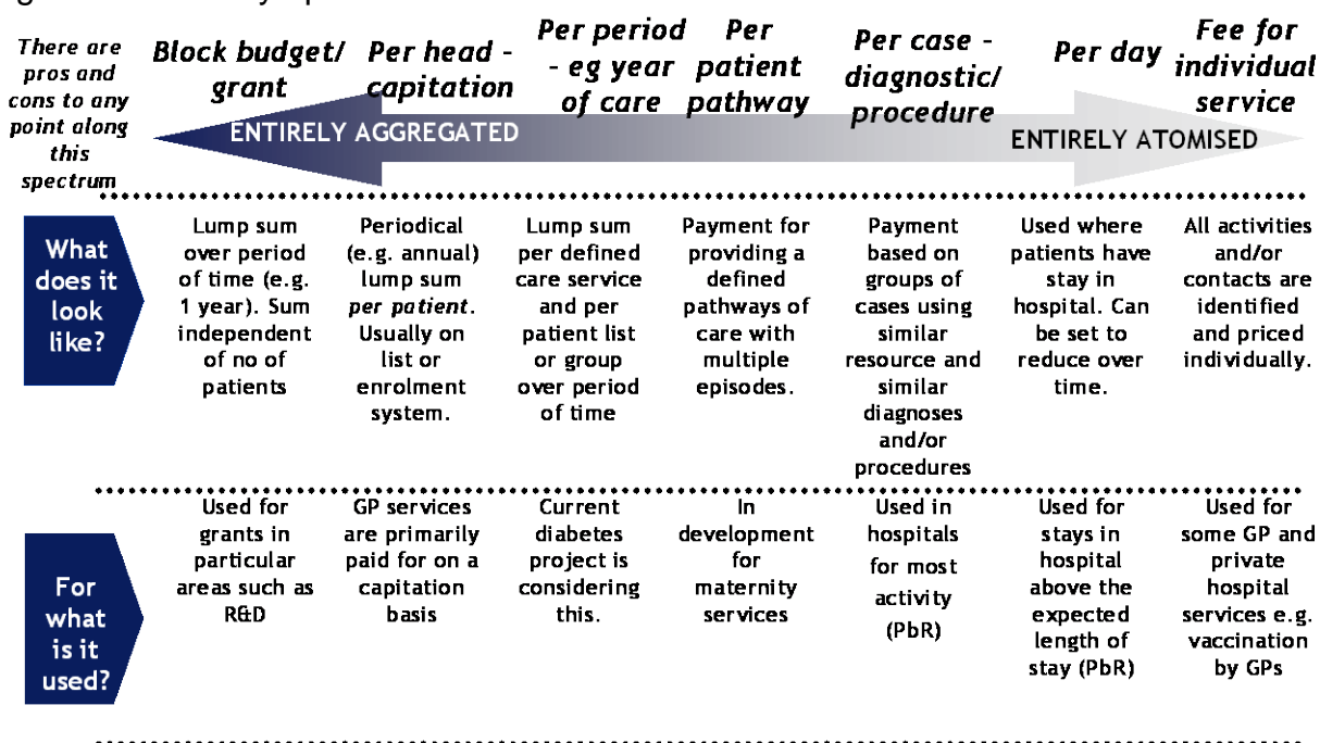
Figure 8: Currency options
